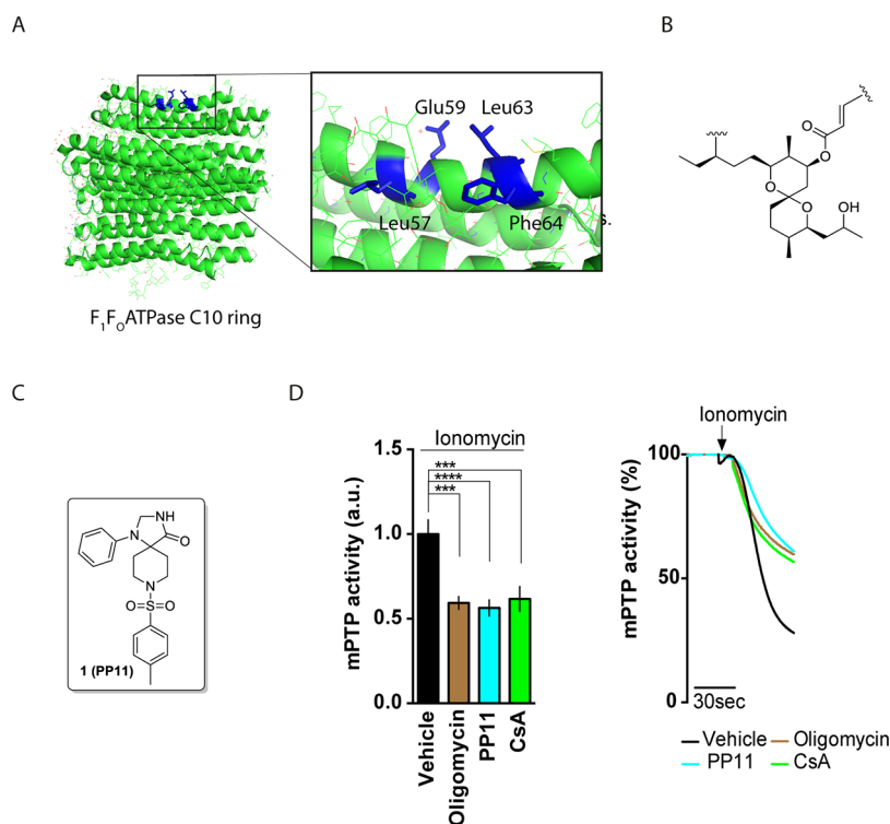
Figure 1. Discovery of PP11 as the first small-molecule inhibitor of the mPTP with a spirocenter template that mimics the spiroketal moiety of oligomycin A. (A) Graphical representation of the key amino acid residues defining the binding pocket of the known mPTP inhibitor oligomycin A to the c ring. (B) Structure of the southern portion of oligomycin A showing a 1,7-dioxaspiro[5.5]undecan moiety that is closely involved in the interaction with the c ring. (C) Structure of PP11, a novel small-molecule inhibitor of the mPTP with a 1,3,8-triazaspiro[4.5]decan-4-one template. (D) Calcein–cobalt assay in living cells pretreated with vehicle, oligomycin A, PP11, and CsA. mPTP opening was stimulated by ionomycin administration, and representative kinetics data are reported. (***) p value < 0.001. (***) p value < 0.0001. CsA: cyclosporine A.
