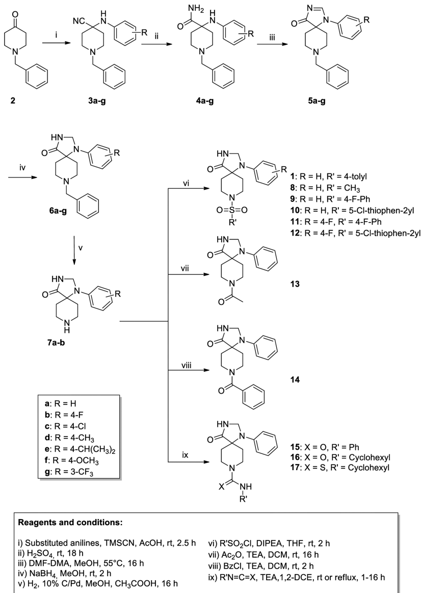
Figure 3. Synthesis of PP11 and related spiro bicyclic derivatives.
